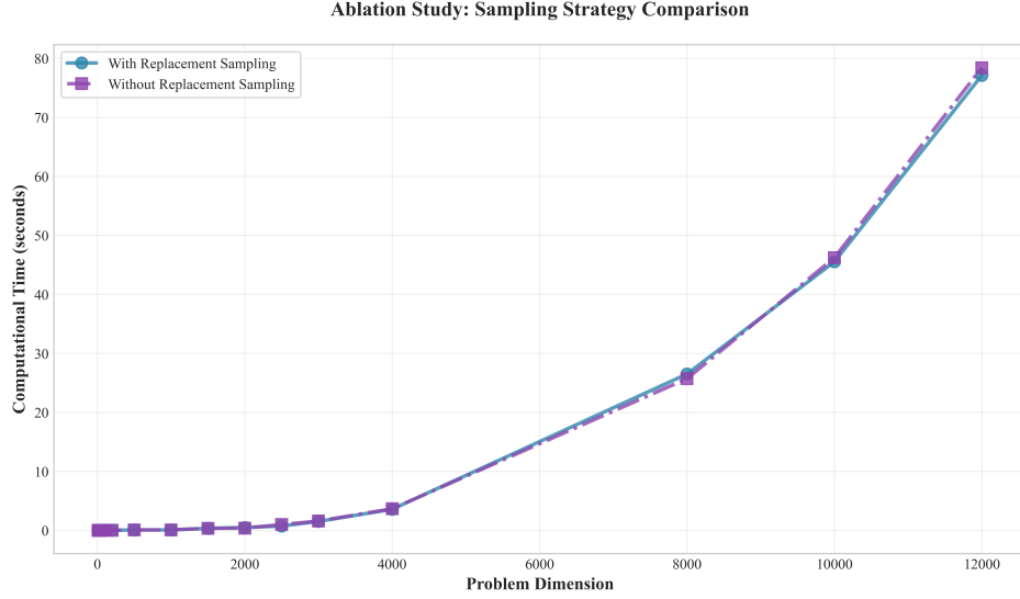
Figure 4: Comparison of sampling strategies showing computational time. Both strategies achieve comparable performance, validating the use of simpler with-replacement sampling in practical implementations.
