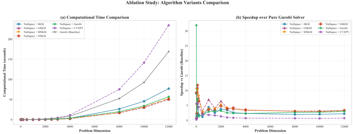
Figure 5: Comparison of algorithmic variants showing computational time (left) and speedup over pure Gurobi solver (right). Momentum-enhanced SKM variants achieve superior performance compared to traditional optimization methods within the nullspace framework.
